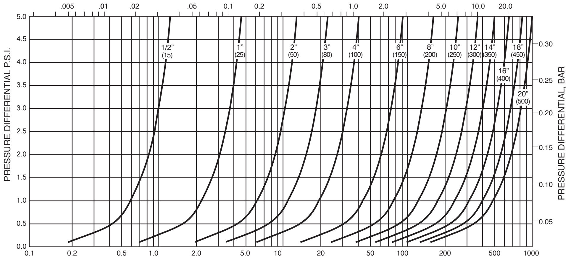
FLOW OF AIR THRU AN ORIFICE IN S.C.F.S. (STANDARD CUBIC FEET OF FREE AIR PER SECOND)
